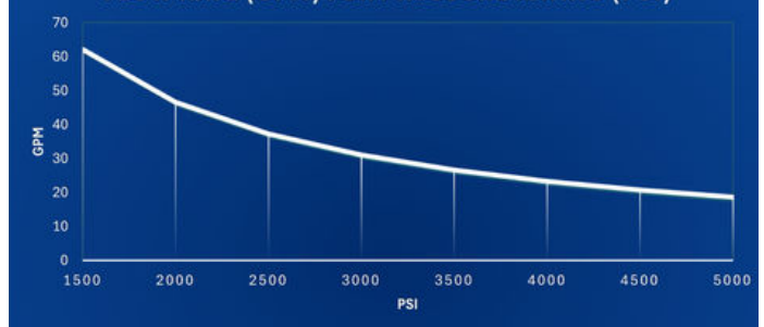
FLOW RATE (GPM) PER PRESSURE RATING (PSI)
